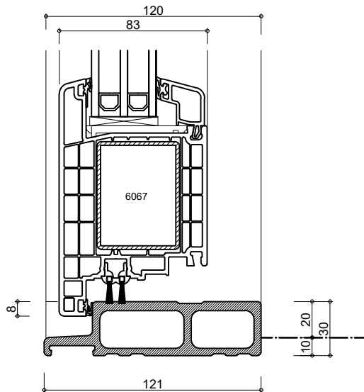
IsoStone dorpel PS0680
