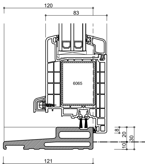
IsoStone dorpel PS0530
