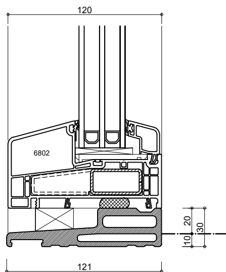
IsoStone dorpel PS0530
